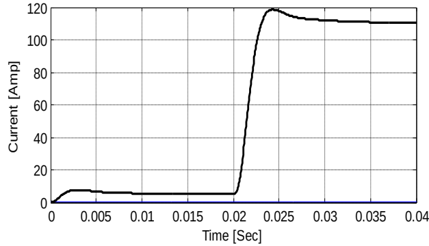
Fig.11 Fault bus current without protection.
