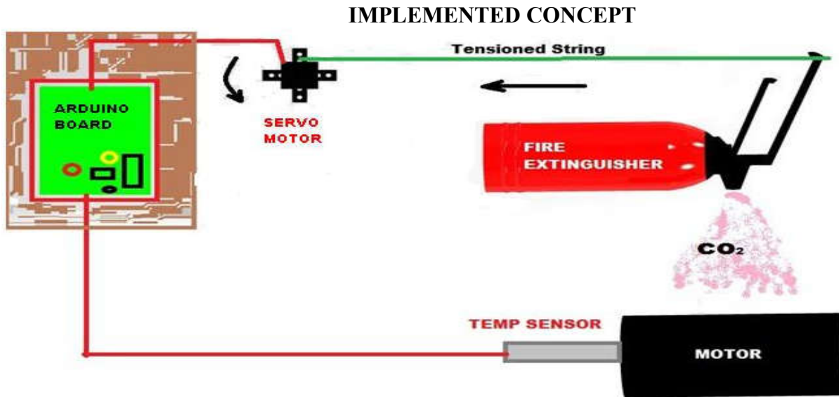
Diagram of Automatic Fire Extinguisher in our Kart
