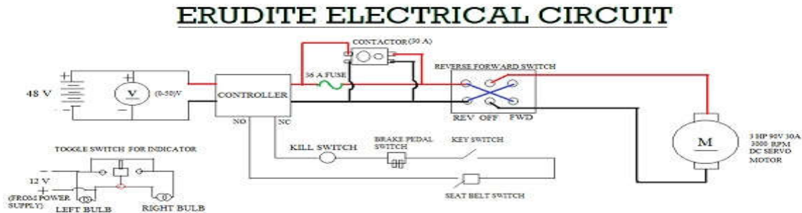
Fig 3 . Kart Electrical Circuit Diagram
