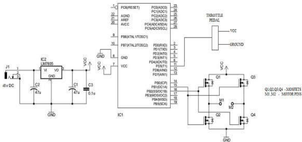
Fig 2 . Kart Controller and Driver Circuit Diagram
