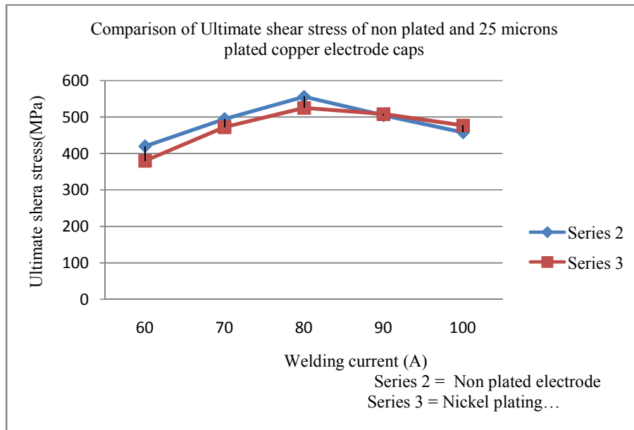
Fig 7.4: Effect of welding current and 25 microns plating on ultimate shear strength.
