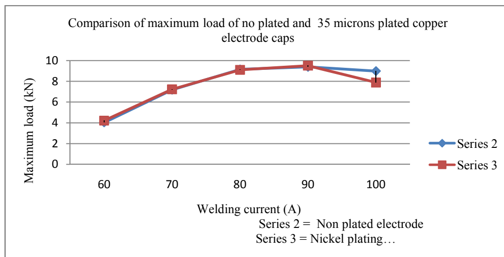
Fig 7.5: Effect of welding current and 35 microns plating on maximum load carrying capacity.
