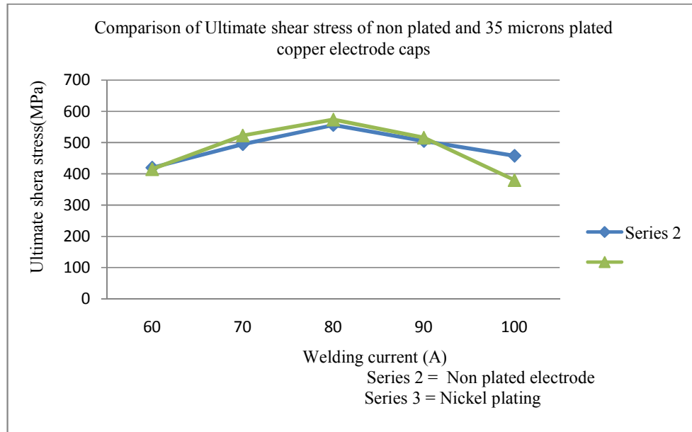
Fig 7.6: Effect of welding current and 35 microns plating on ultimate shear strength.
