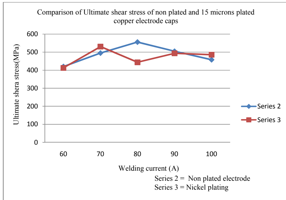
Fig 7.2 : Effect of welding current and 15 microns plating on ultimate shear strength.
