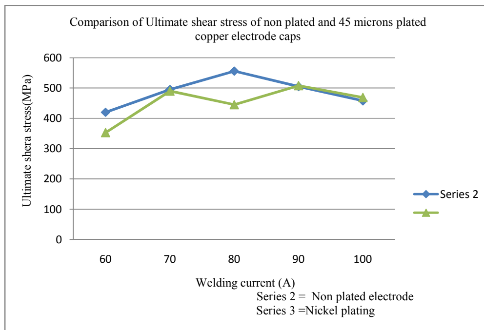
Fig 7.8: Effect of welding current and 45 microns plating on maximum load carrying capacity.
