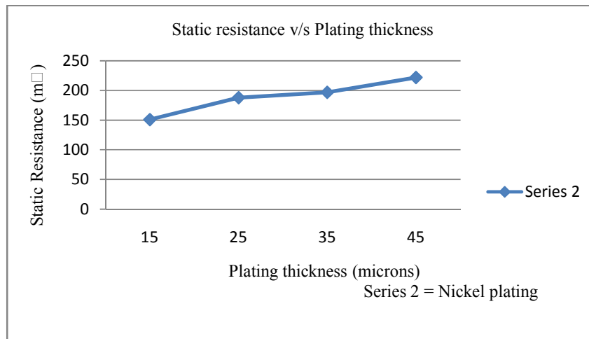
Fig 6.1: Effect of plating thickness on static resistance of the weld system.
