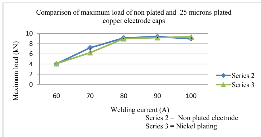
Fig 7.3 : Effect of welding current and 25 microns plating on maximum load carrying capacity.
