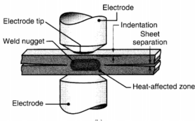
Fig 1.1: Cross section of a spot weld, showing the weld nugget and the indentation of the electrode on the sheet surfaces.
