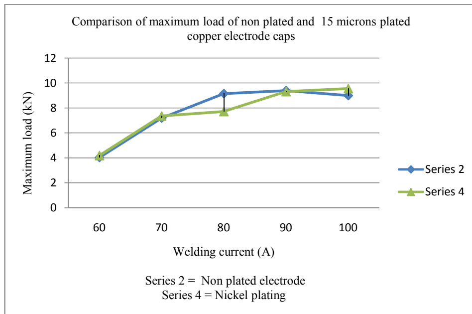
Fig 7.1: Effect of welding current and 15 microns plating on maximum load carrying capacity.
