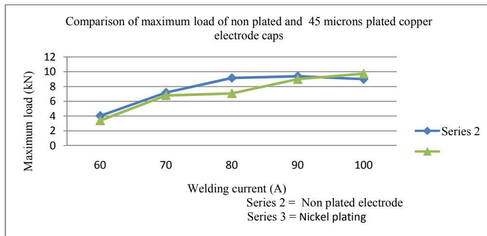
Fig 7.7: Effect of welding current and 45 microns plating on maximum load carrying capacity.
