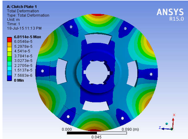
Figure 5: Total deformation in Clutch Plate 1
