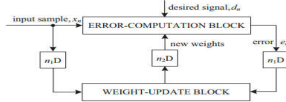
Fig. 1. Structure of the conventional delayed LMS adaptive filter
