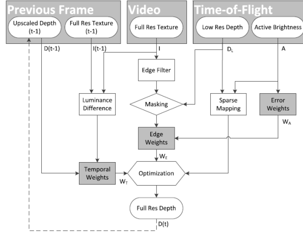
Fig.9: EWOC Framework.
