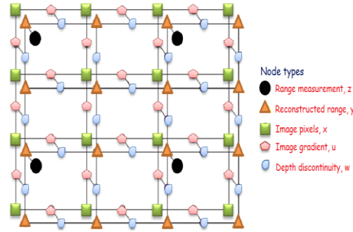
Fig.7: MRF Framework.
