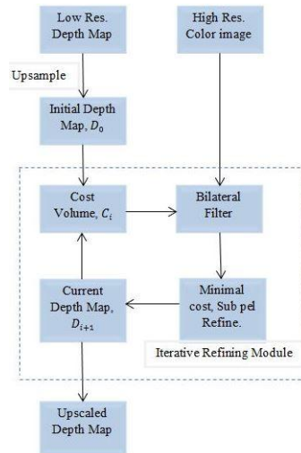
Fig.8: JBU Framework.
