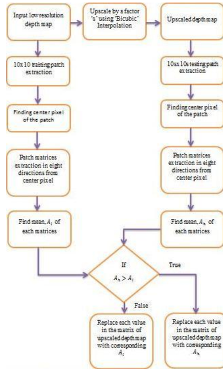
Fig.11: Patch Match algorithm Flow Chart.
