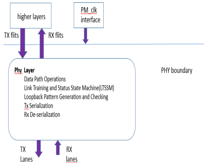
Fig. 3. Interconnect IP
