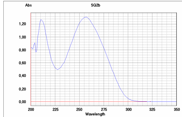
Figure 8. Wavelength spectrum of chromosomal DNA of strain SQ2b
