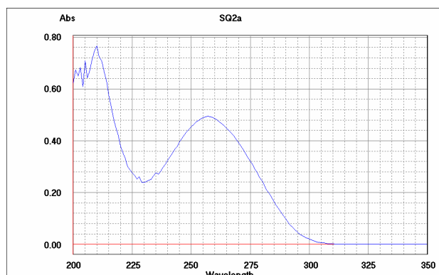
Figure 7. Wavelength scan spectrum of chromosomal DNA of strain SQ2a
