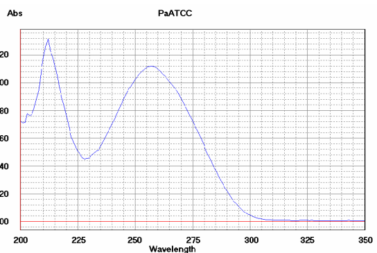
Figure 6. Wavelength scan spectrum of chromosomal DNA of strain Pseudomonas aeruginosa ATCC 27853
